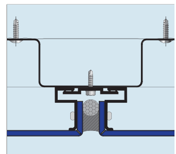
ALUCOFIX INSTALLATION
