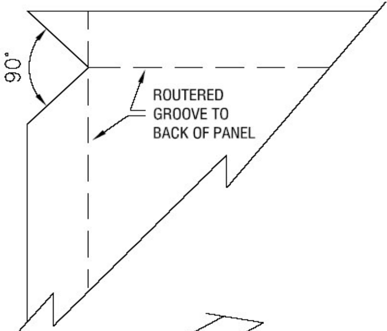
DETAIL OF CUT-OUT TO CORNER
